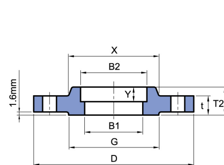
SOCKET WELDING
